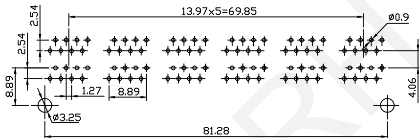
PCB Layout
